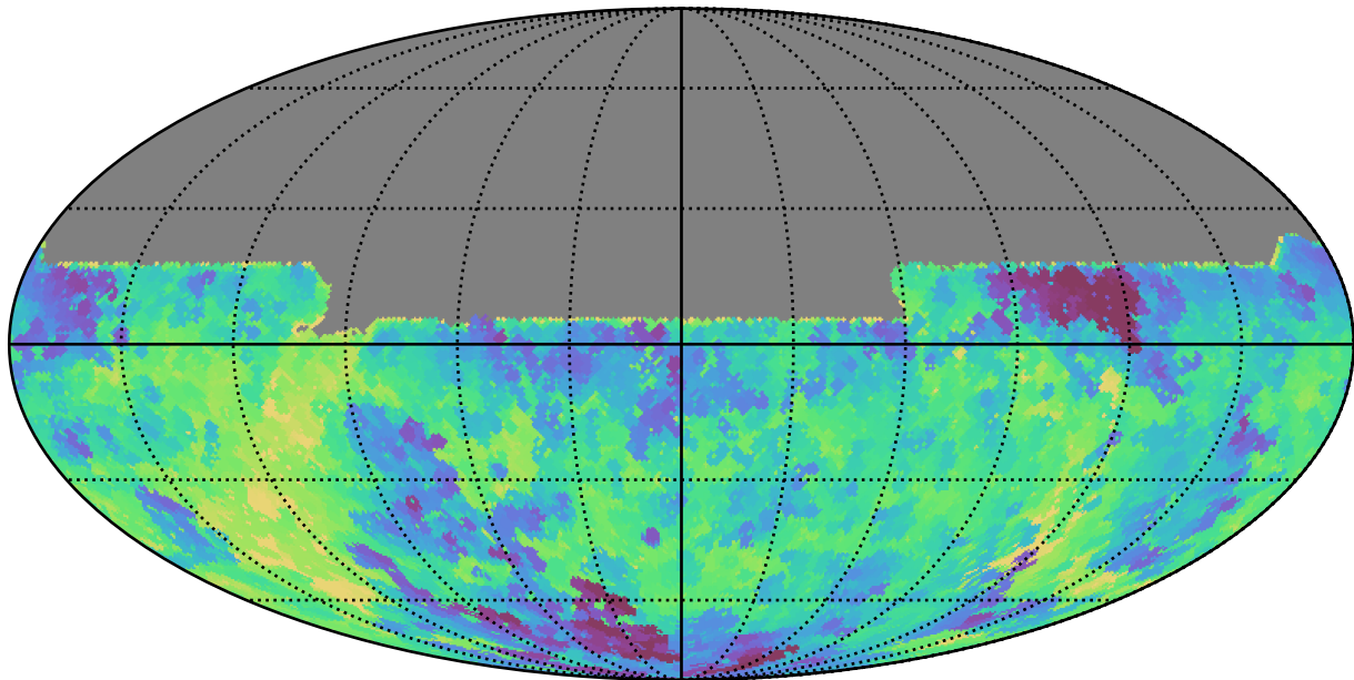
too_5_1v3.4_10yrs All sky u band: Min fiveSigmaDepth
