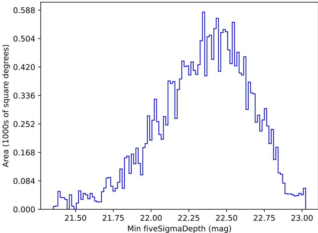
too_5_1v3.4_10yrs All sky u band: Min fiveSigmaDepth
