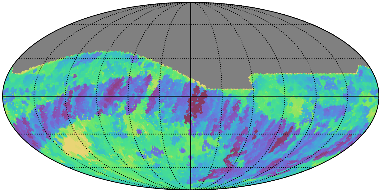
too_5_1v3.4_10yrs All sky r band: Min fiveSigmaDepth
