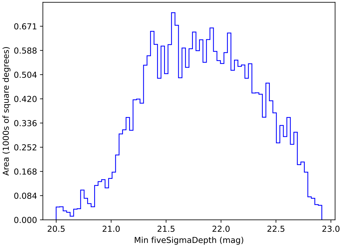
too_5_1v3.4_10yrs All sky i band: Min fiveSigmaDepth
