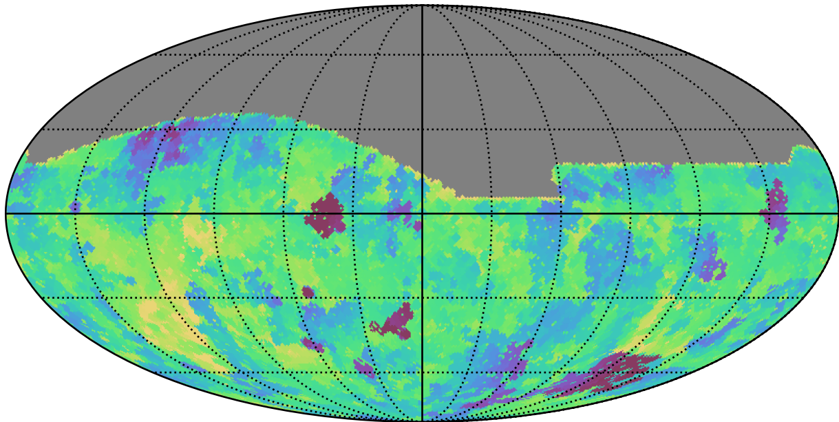
too_5_1v3.4_10yrs All sky g band: Min fiveSigmaDepth
