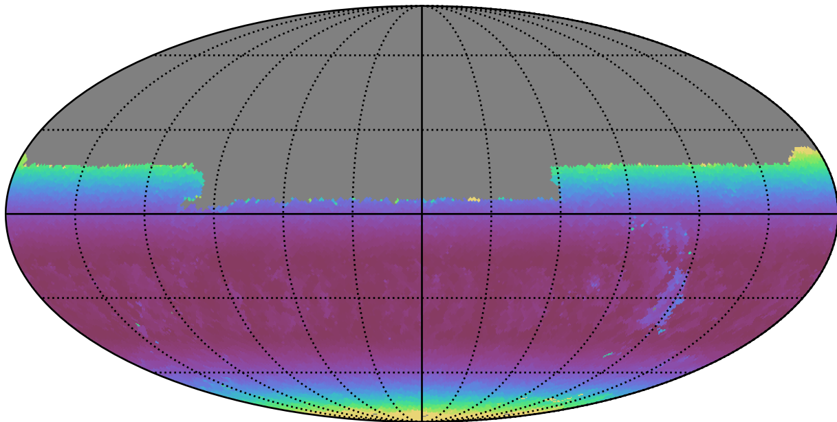
too_5_1v3.4_10yrs Yr 1 y band: Min airmass
