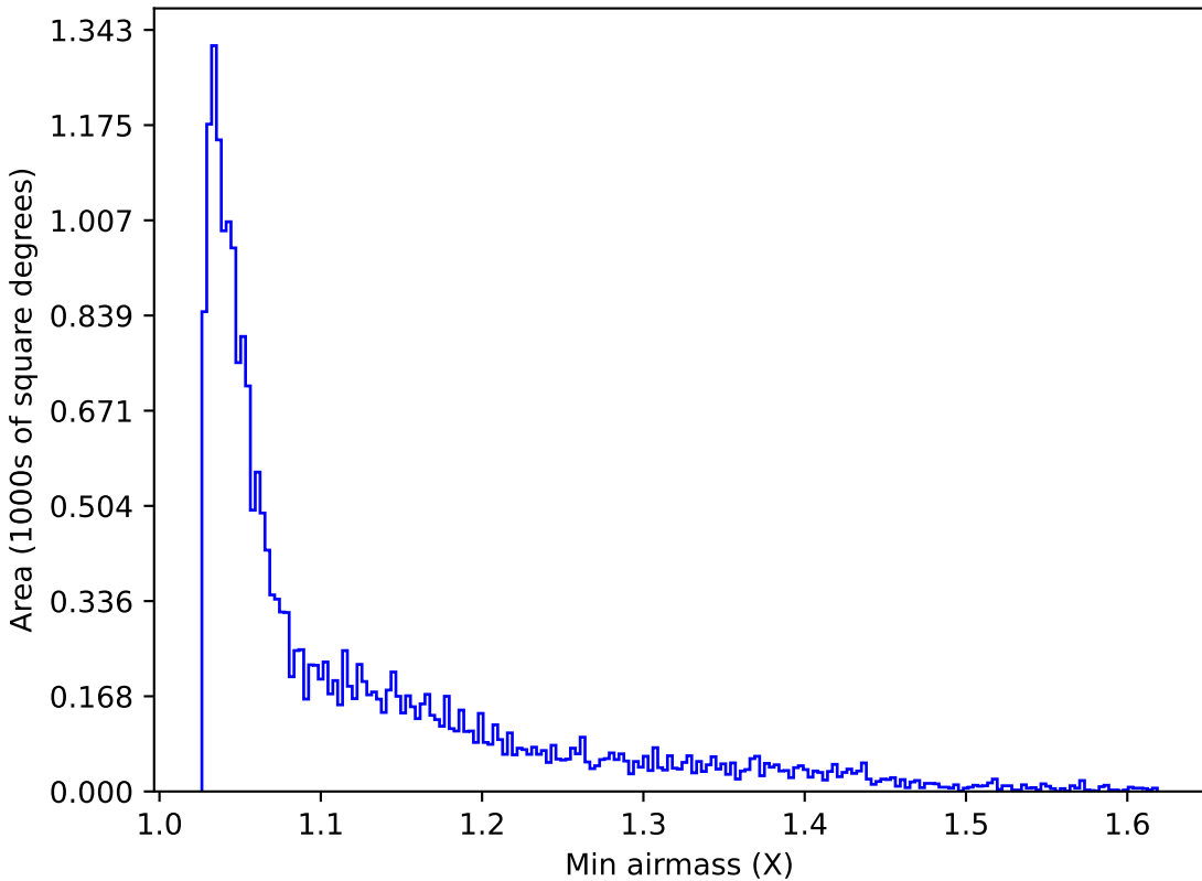
too_5_1v3.4_10yrs Yr 1 y band: Min airmass
