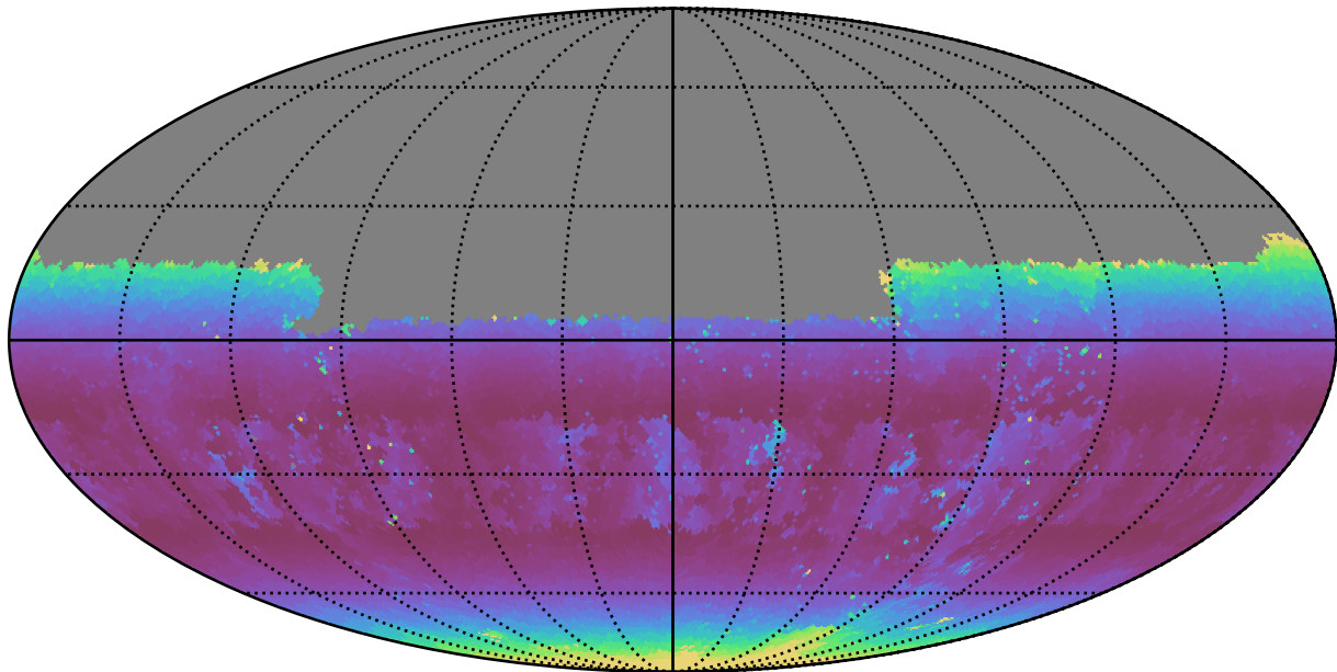
too_5_1v3.4_10yrs Yr 1 u band: Min airmass
