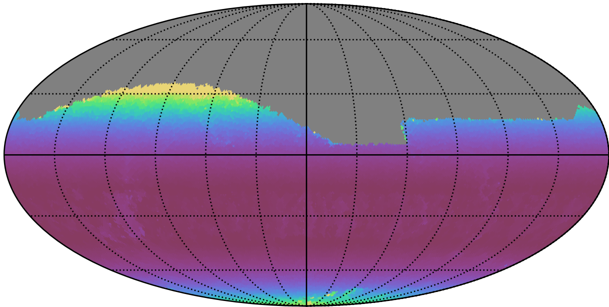
too_5_1v3.4_10yrs Yr 1 r band: Min airmass
