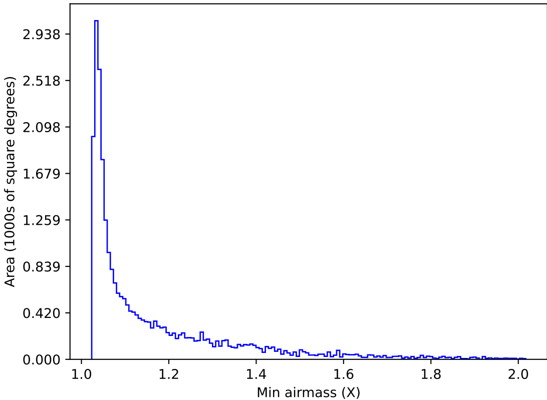
too_5_1v3.4_10yrs Yr 1 r band: Min airmass
