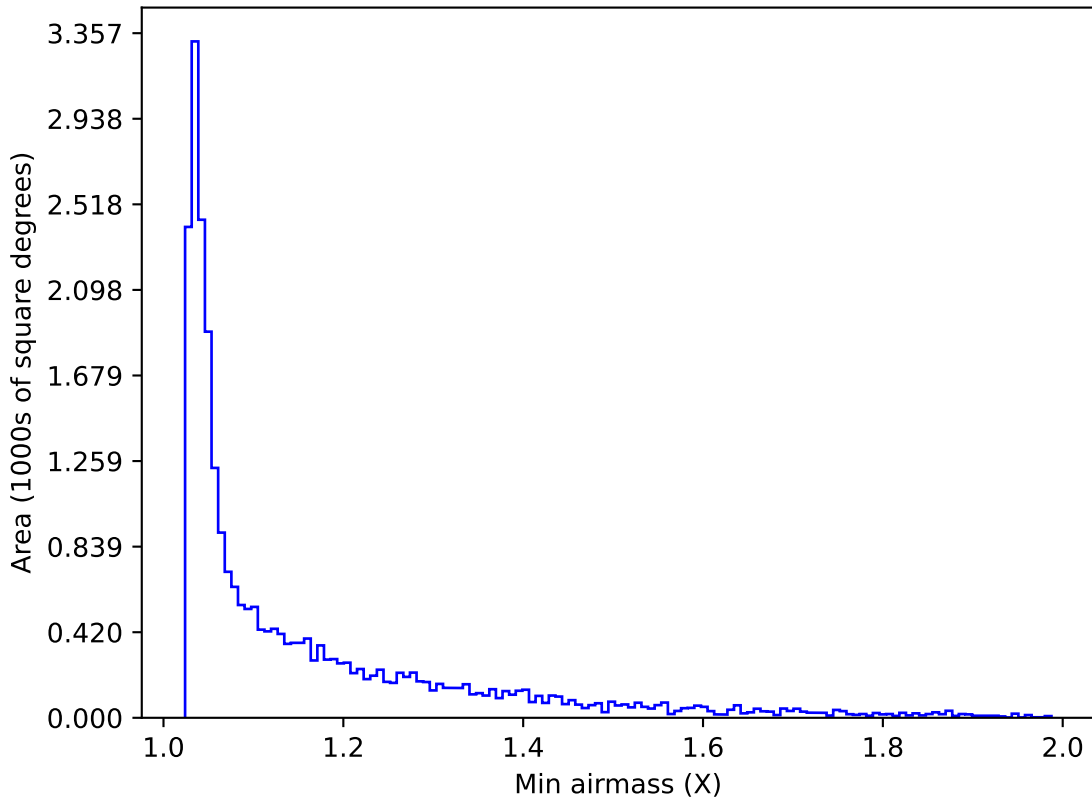
too_5_1v3.4_10yrs Yr 1 i band: Min airmass
