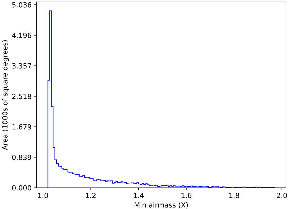
too_5_1v3.4_10yrs Yr 1 all bands: Min airmass
