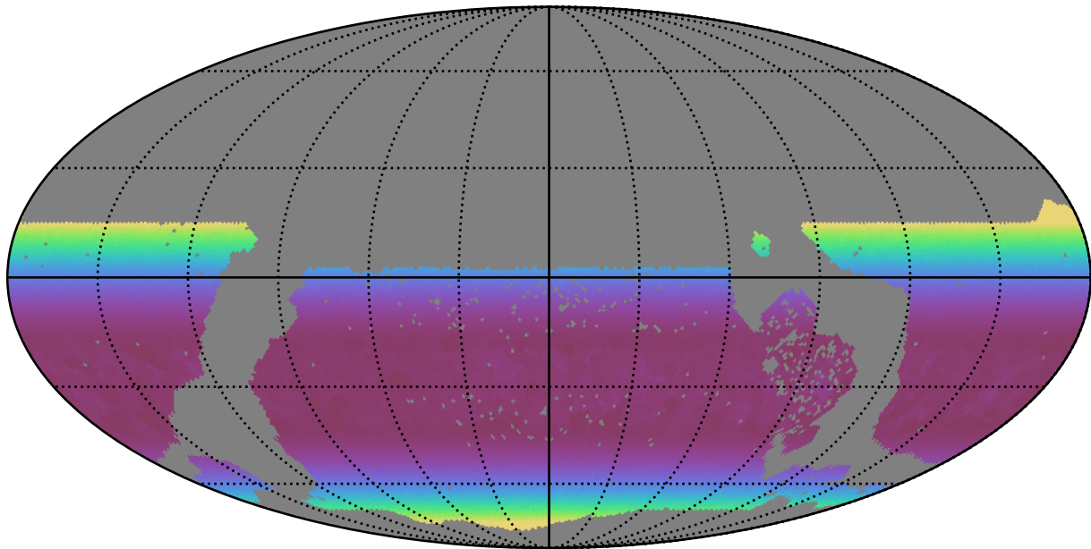
too_5_1v3.4_10yrs WFD z band: Min airmass
