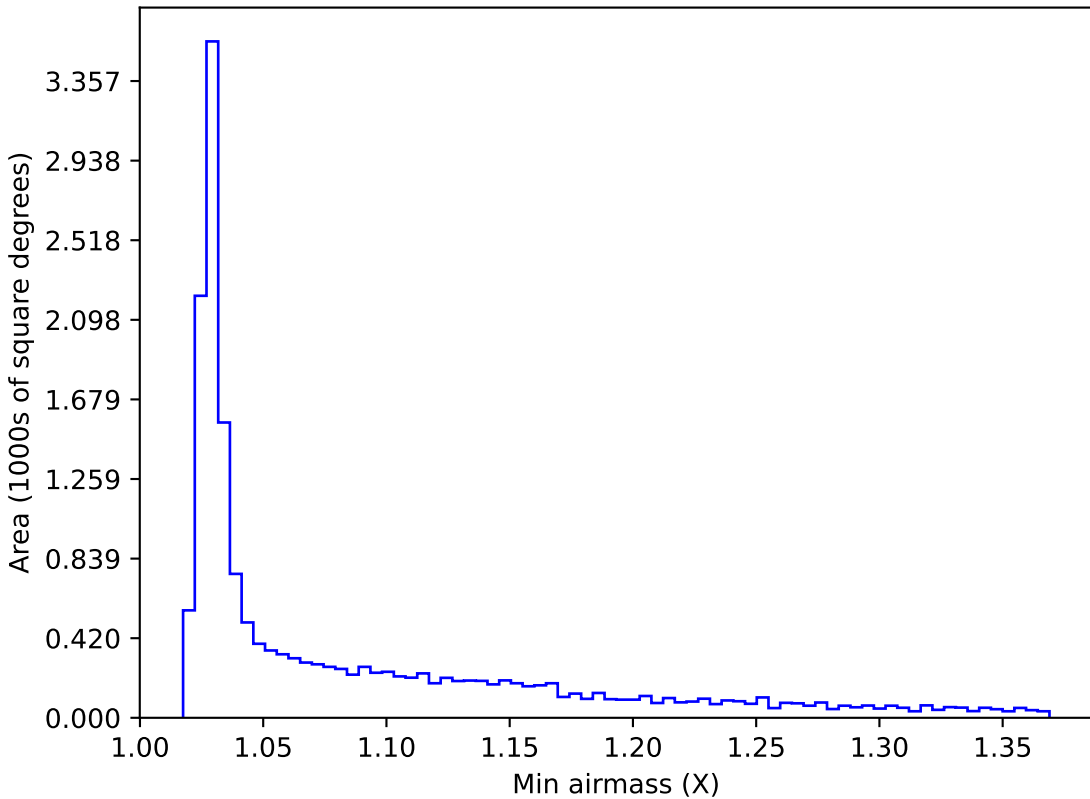
too_5_1v3.4_10yrs WFD z band: Min airmass
