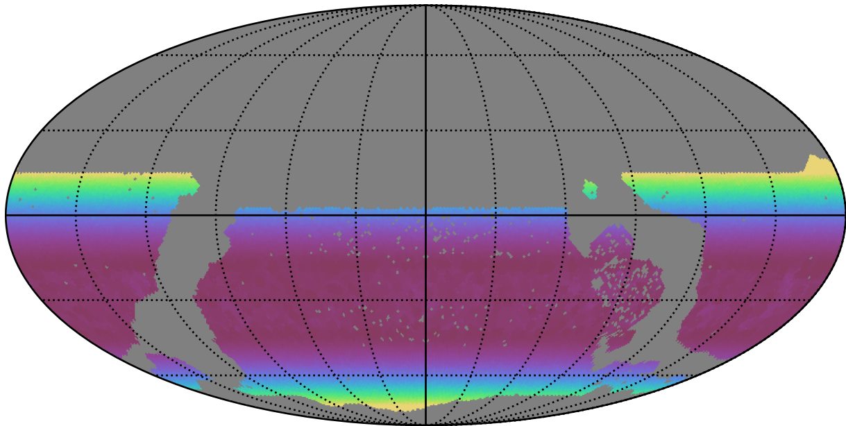
too_5_1v3.4_10yrs WFD y band: Min airmass
