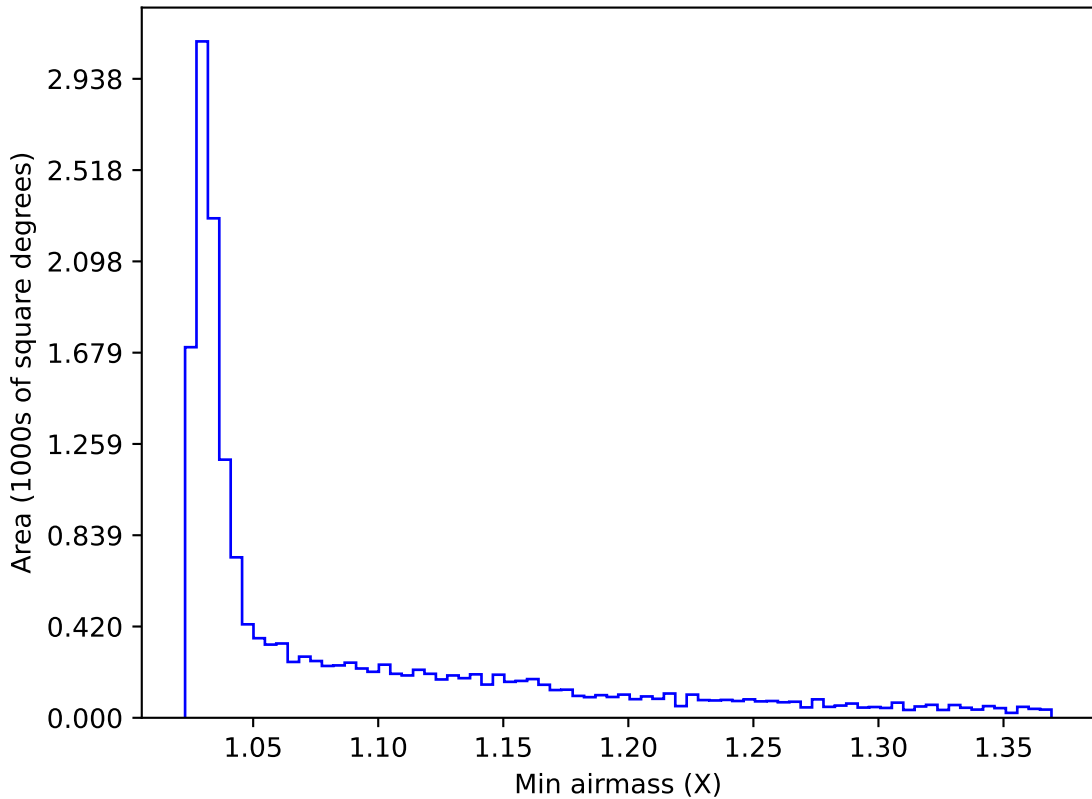
too_5_1v3.4_10yrs WFD y band: Min airmass
