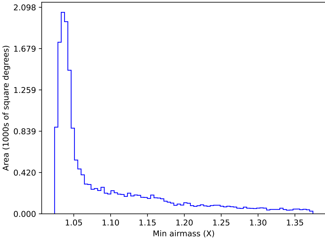
too_5_1v3.4_10yrs WFD u band: Min airmass
