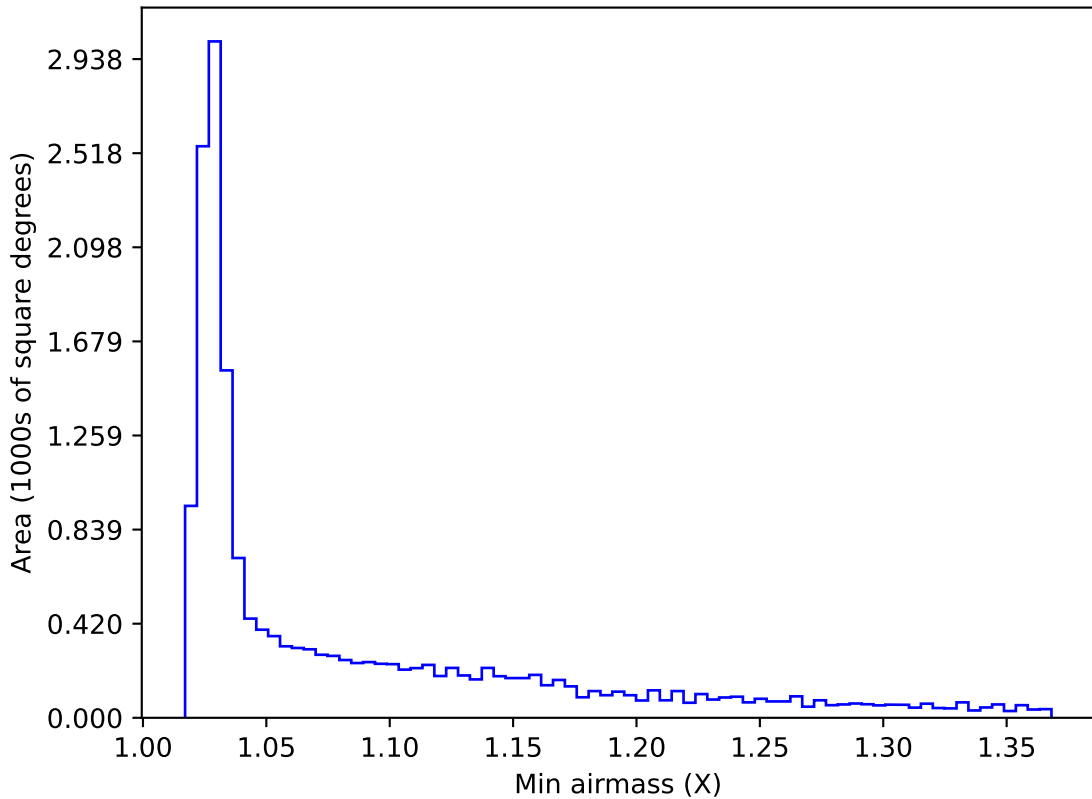
too_5_1v3.4_10yrs WFD r band: Min airmass
