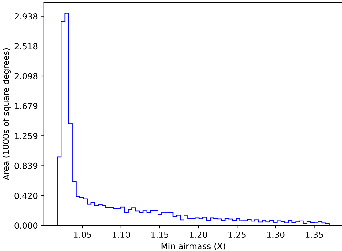
too_5_1v3.4_10yrs WFD i band: Min airmass
