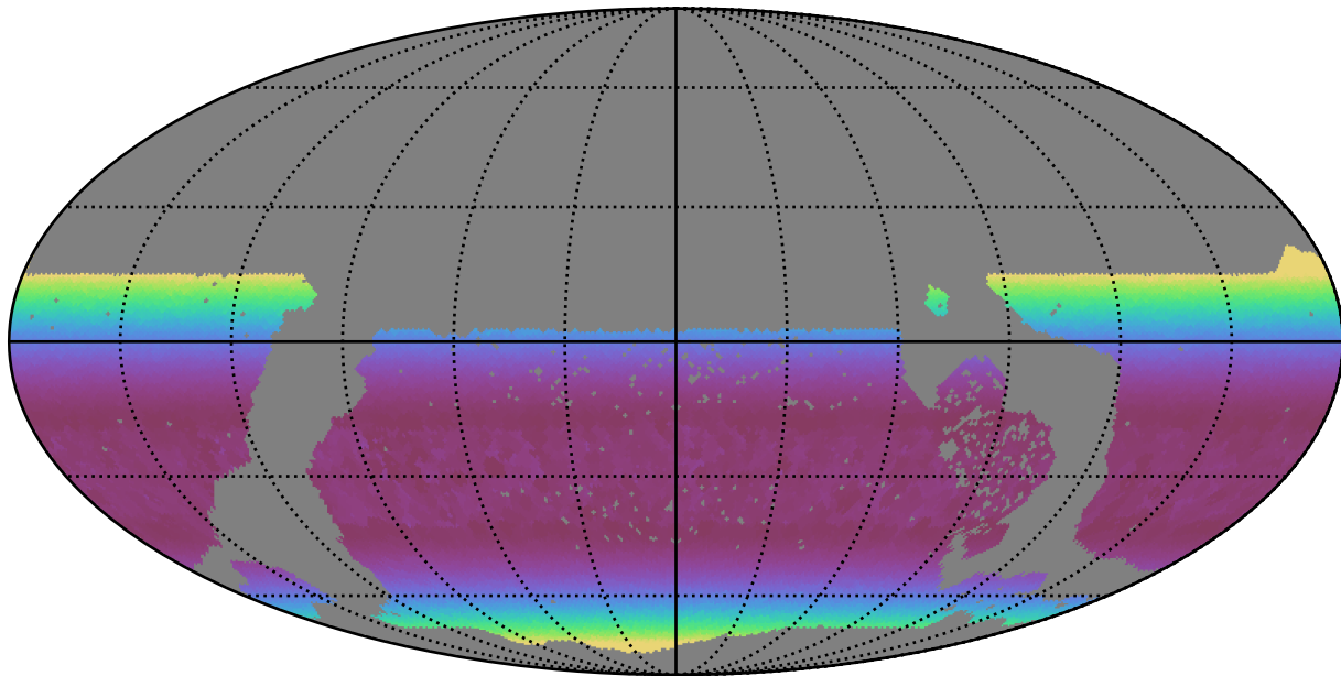
too_5_1v3.4_10yrs WFD g band: Min airmass
