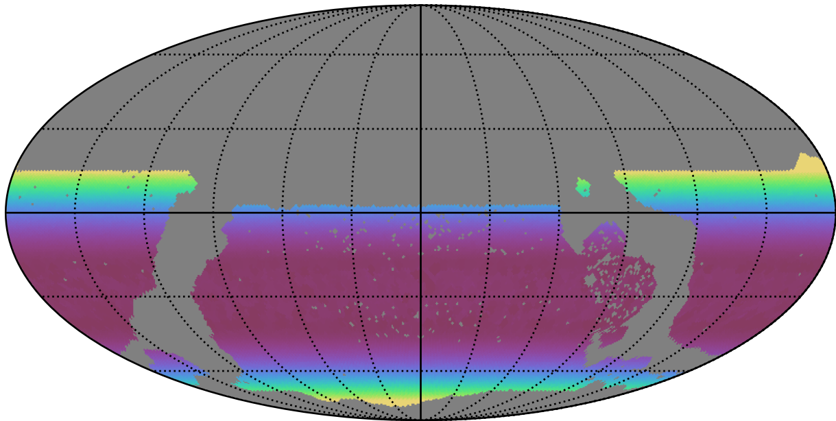
too_5_1v3.4_10yrs WFD all bands: Min airmass
