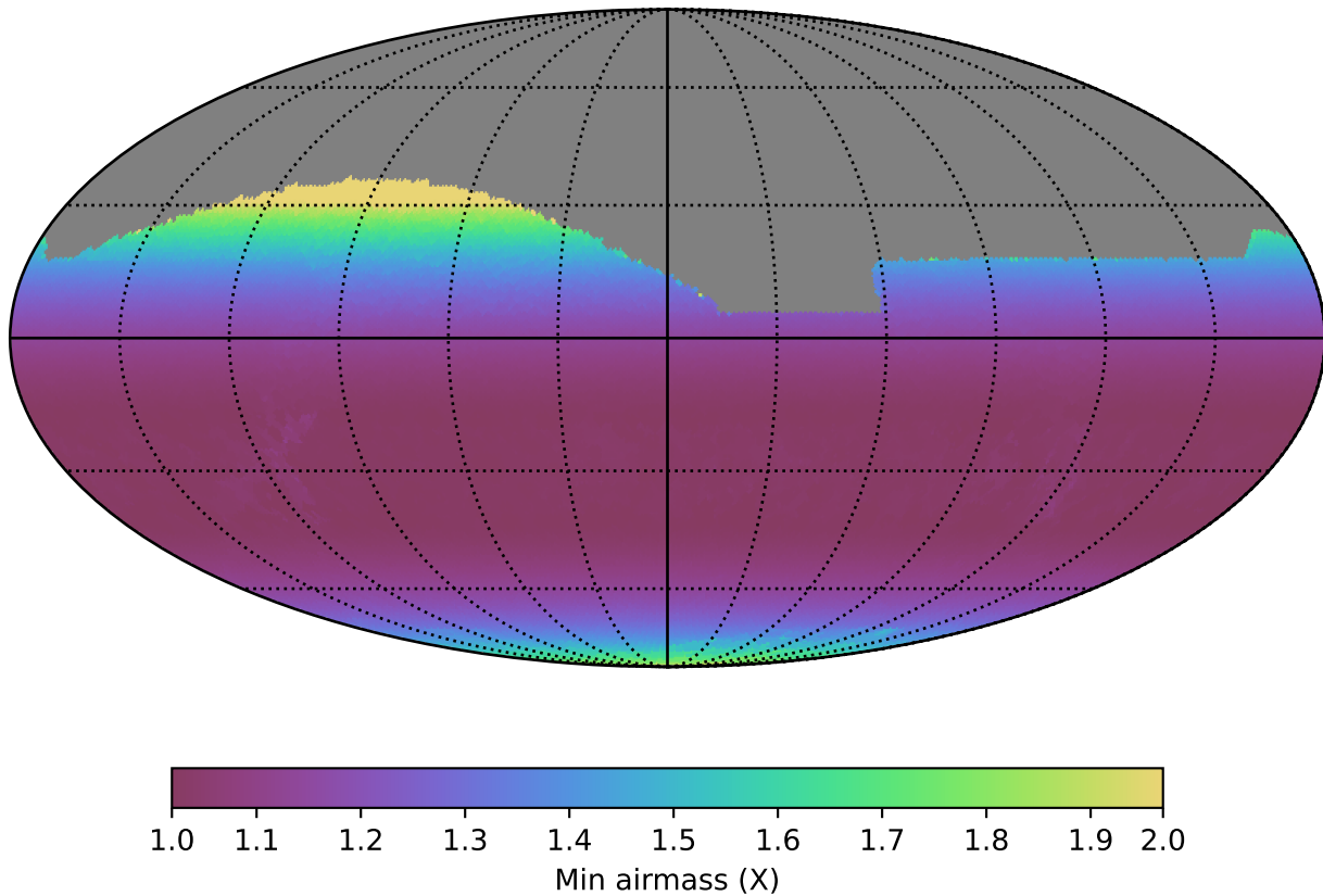
too_5_1v3.4_10yrs All sky z band: Min airmass
