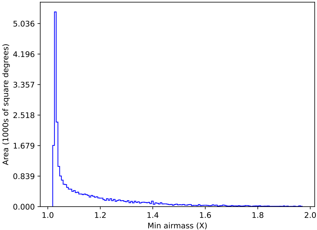
too_5_1v3.4_10yrs All sky z band: Min airmass
