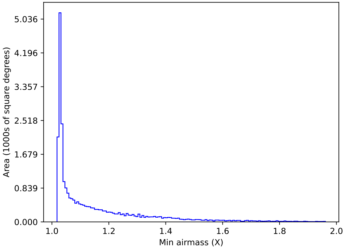
too_5_1v3.4_10yrs All sky i band: Min airmass
