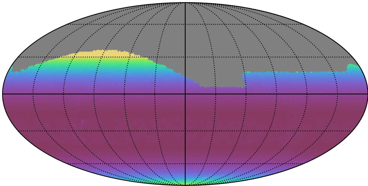
too_5_1v3.4_10yrs All sky g band: Min airmass
