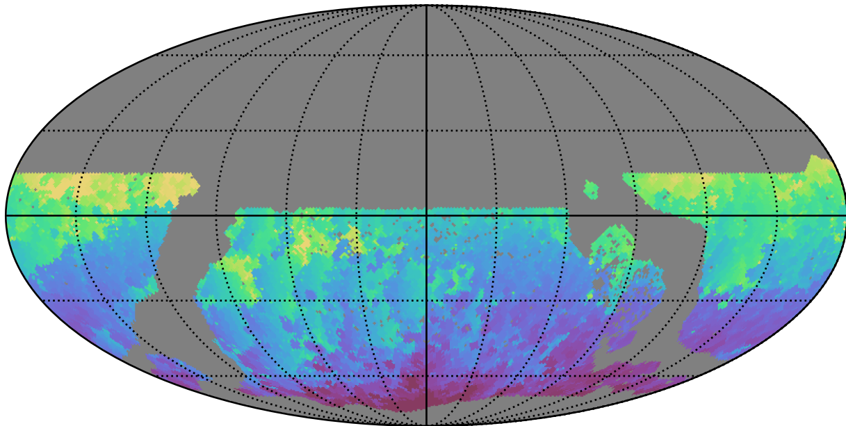
too_5_1v3.4_10yrs WFD z band: Min HA
