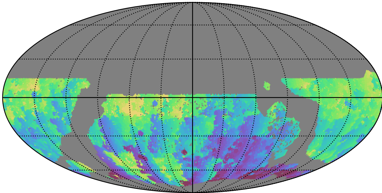
too_5_1v3.4_10yrs WFD u band: Min HA
