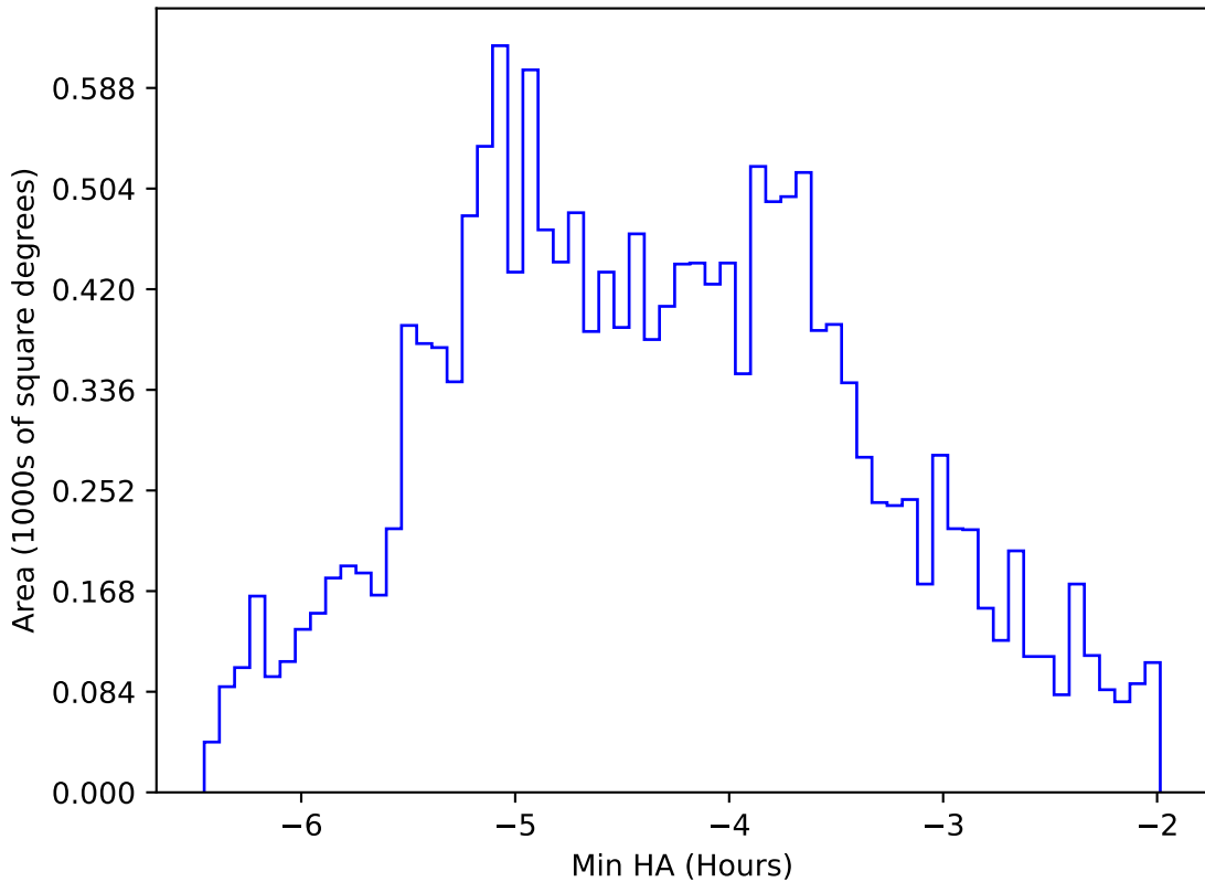
too_5_1v3.4_10yrs WFD i band: Min HA
