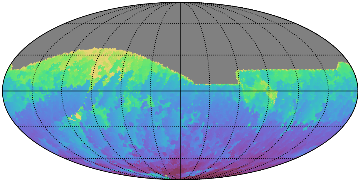
too_5_1v3.4_10yrs All sky z band: Min HA
