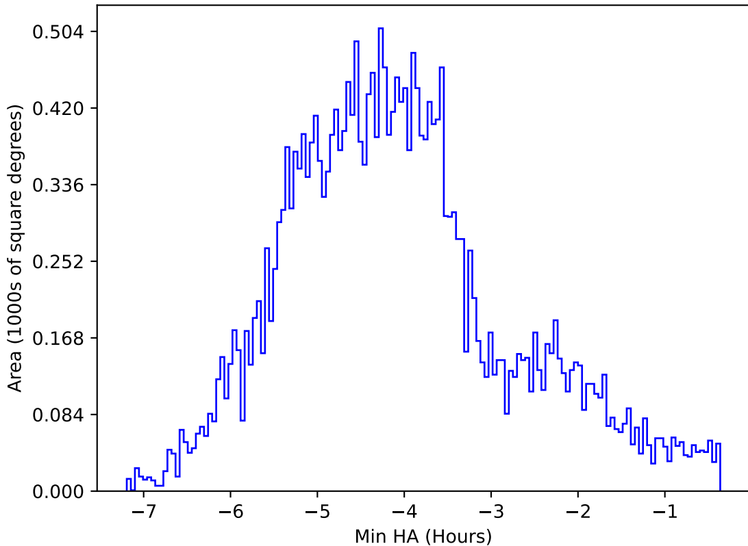
too_5_1v3.4_10yrs All sky z band: Min HA
