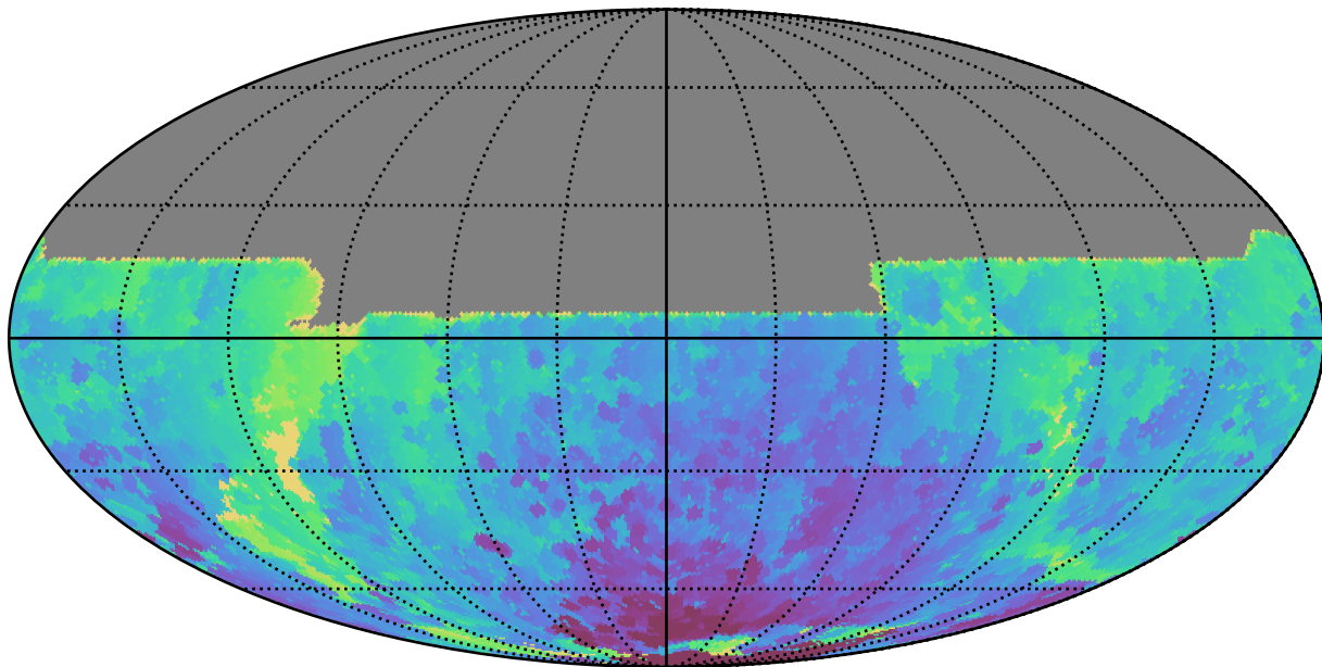
too_5_1v3.4_10yrs All sky y band: Min HA
