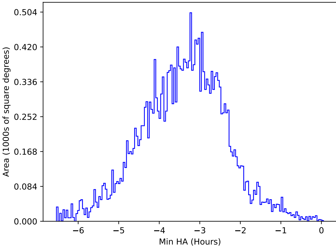
too_5_1v3.4_10yrs All sky y band: Min HA
