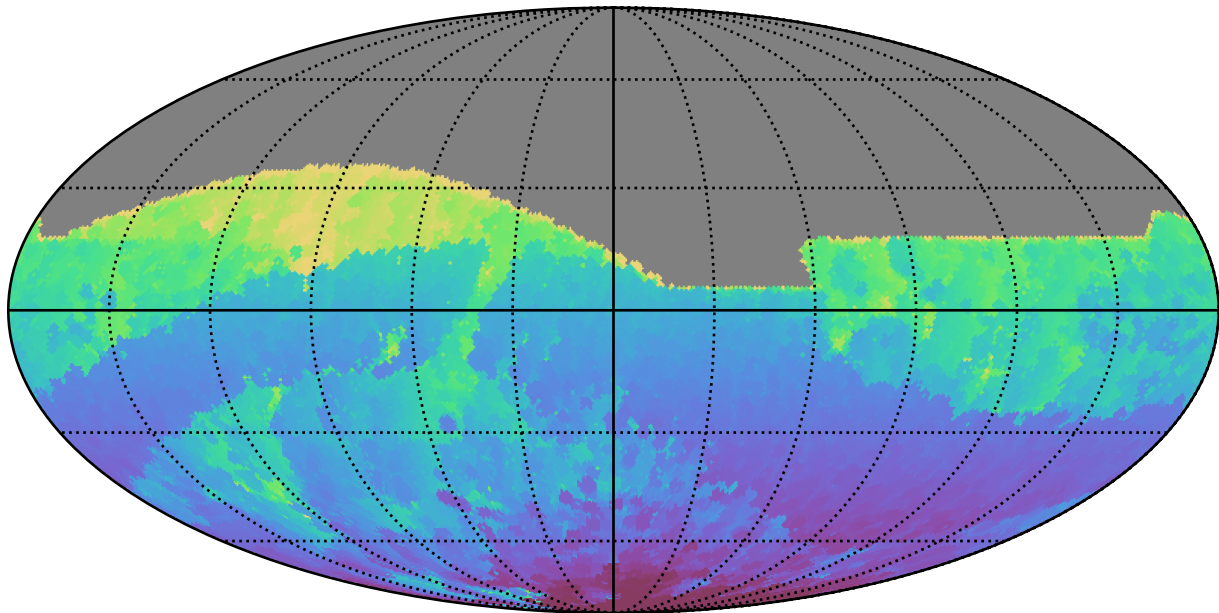
too_5_1v3.4_10yrs All sky r band: Min HA
