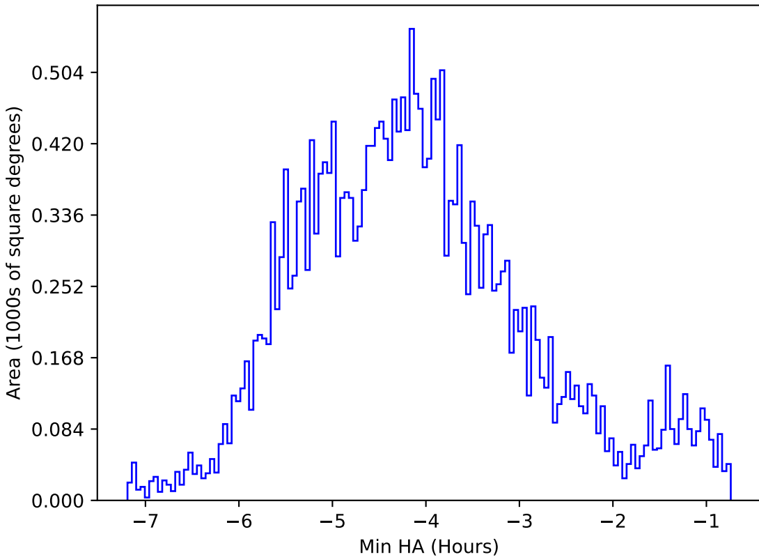
too_5_1v3.4_10yrs All sky r band: Min HA
