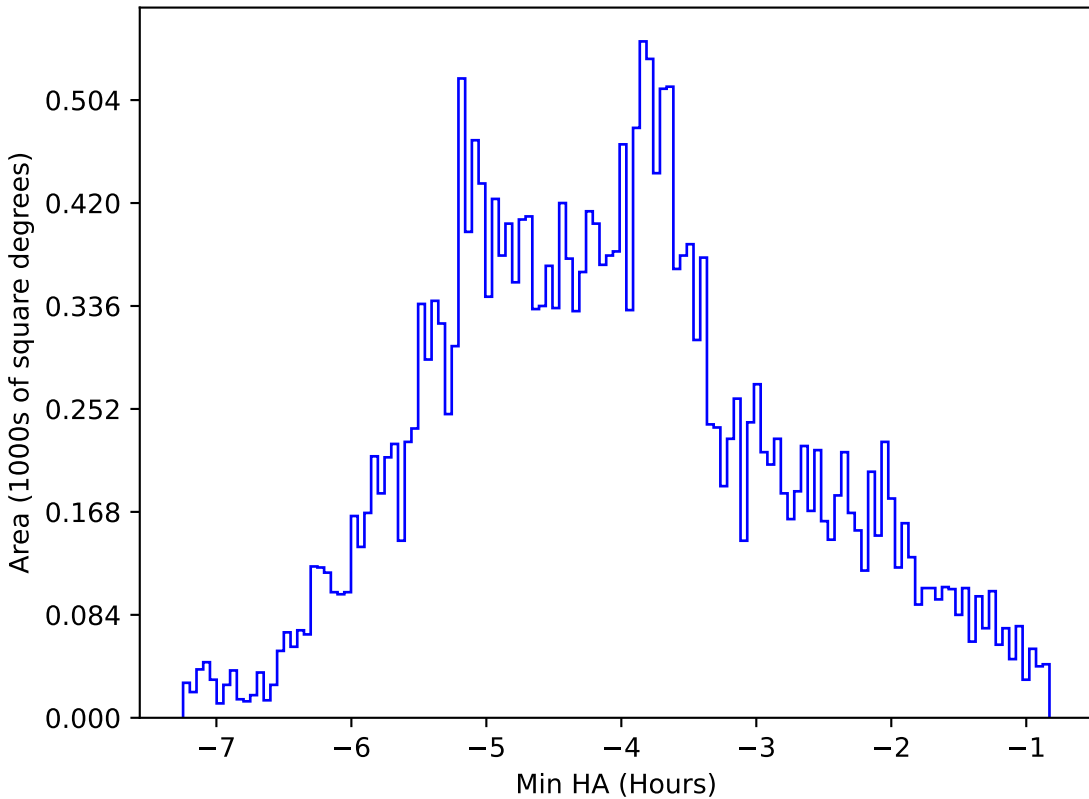
too_5_1v3.4_10yrs All sky i band: Min HA
