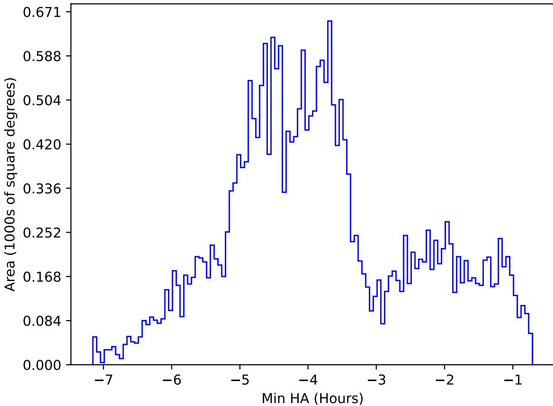
too_5_1v3.4_10yrs All sky g band: Min HA
