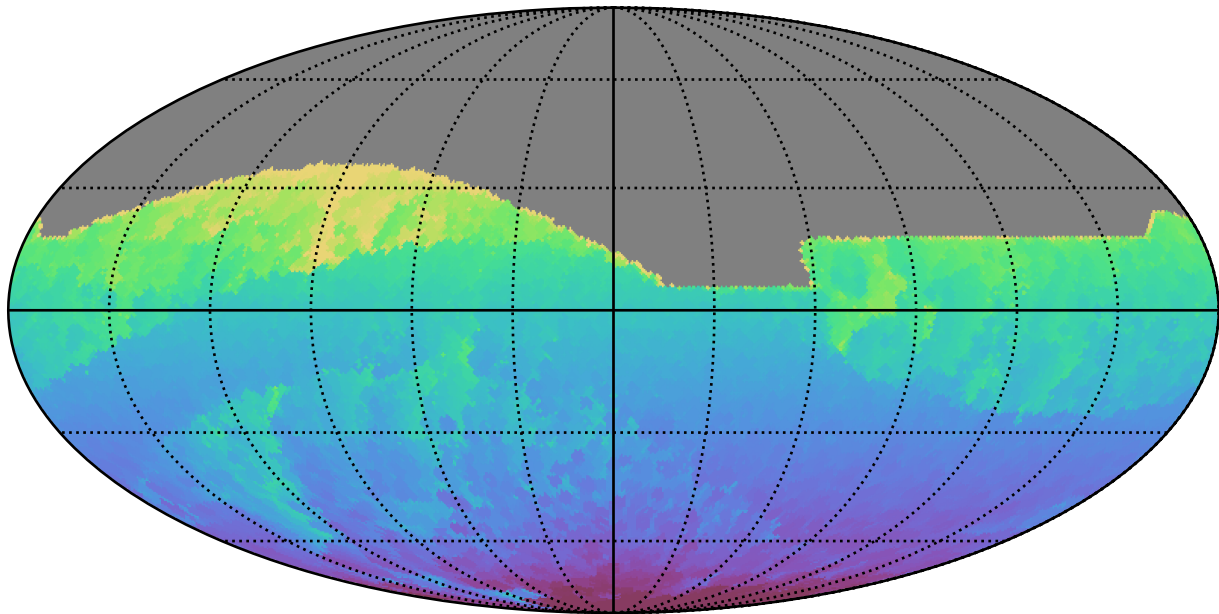
too_5_1v3.4_10yrs All sky all bands: Min HA
