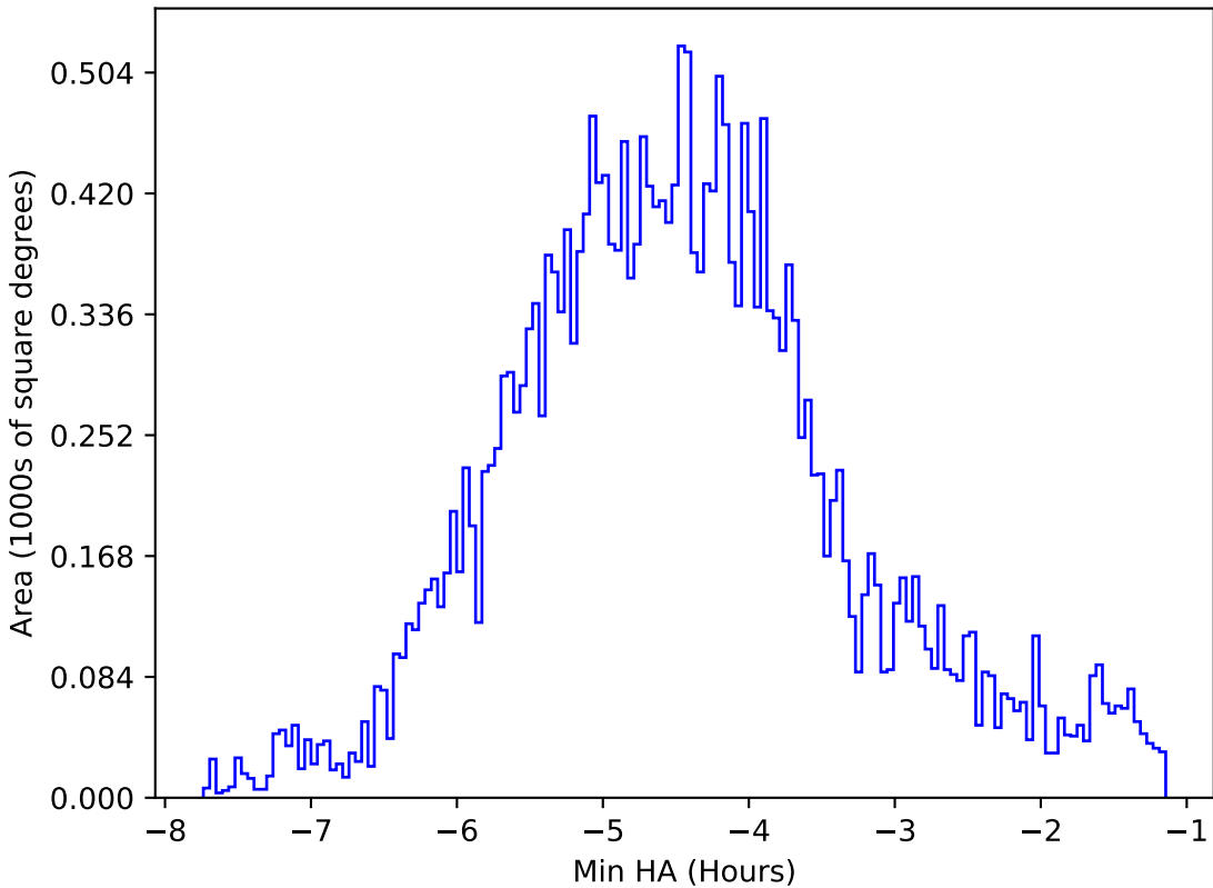
too_5_1v3.4_10yrs All sky all bands: Min HA
