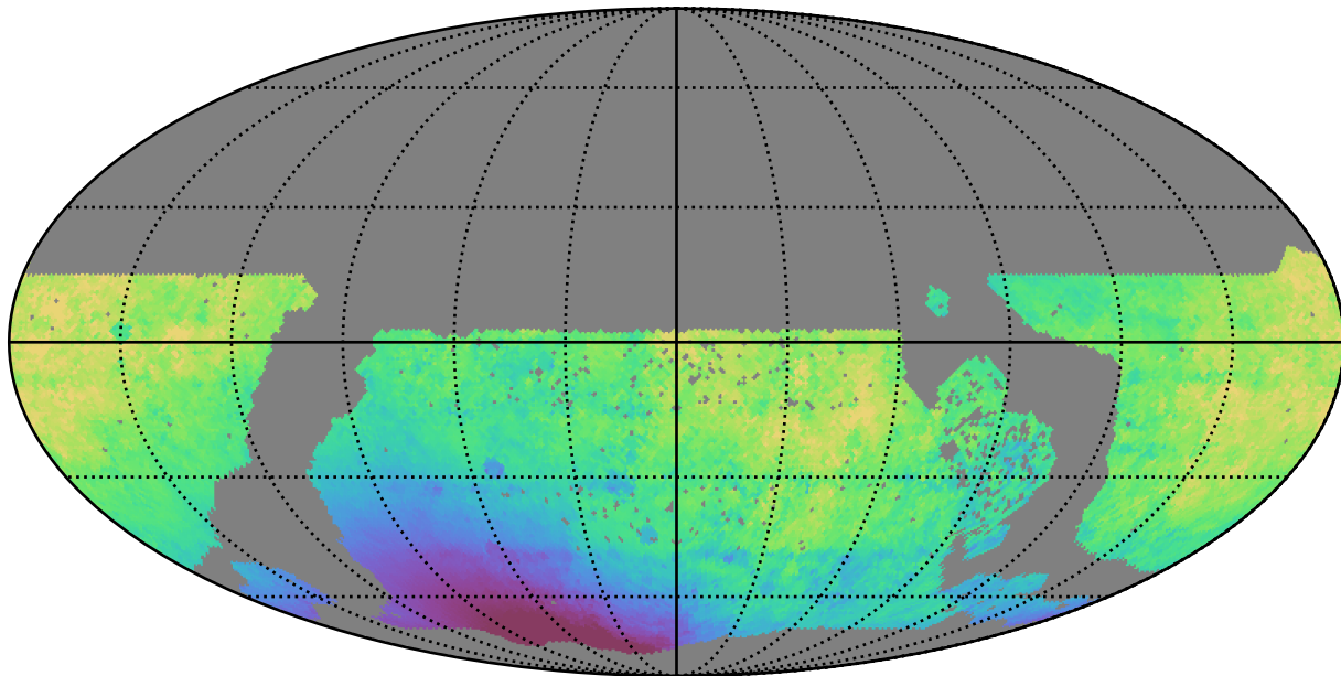
too_5_1v3.4_10yrs WFD z band: Median solarElong
