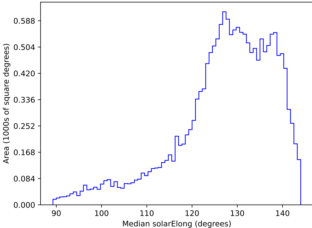
too_5_1v3.4_10yrs WFD z band: Median solarElong
