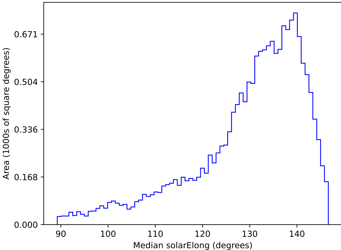
too_5_1v3.4_10yrs WFD y band: Median solarElong
