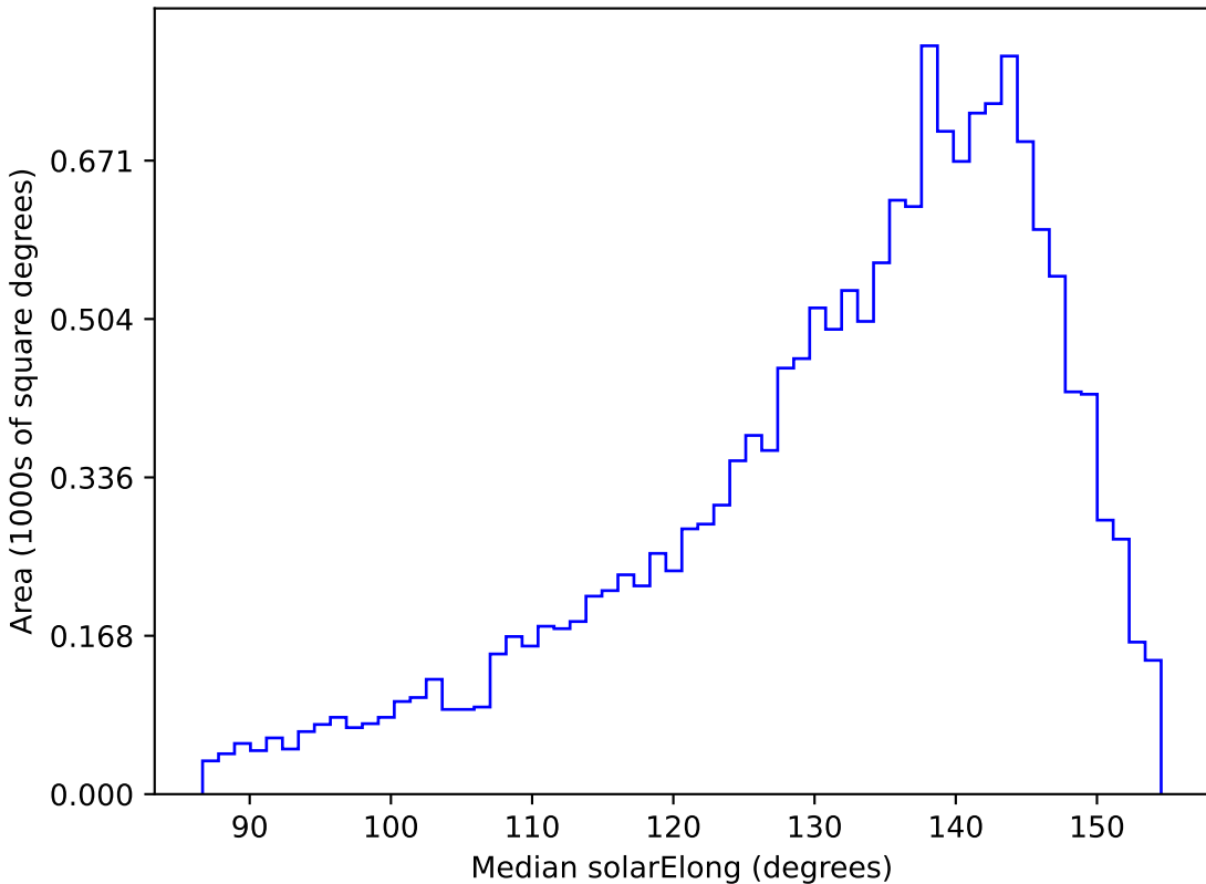
too_5_1v3.4_10yrs WFD u band: Median solarElong
