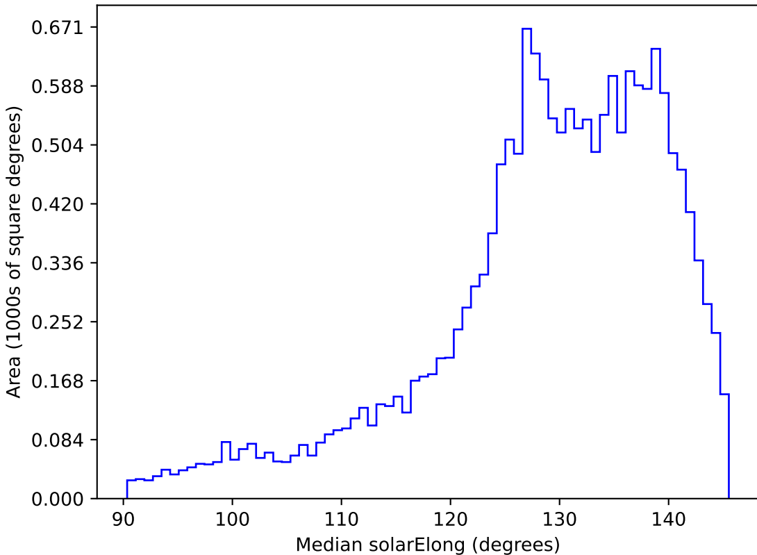
too_5_1v3.4_10yrs WFD i band: Median solarElong
