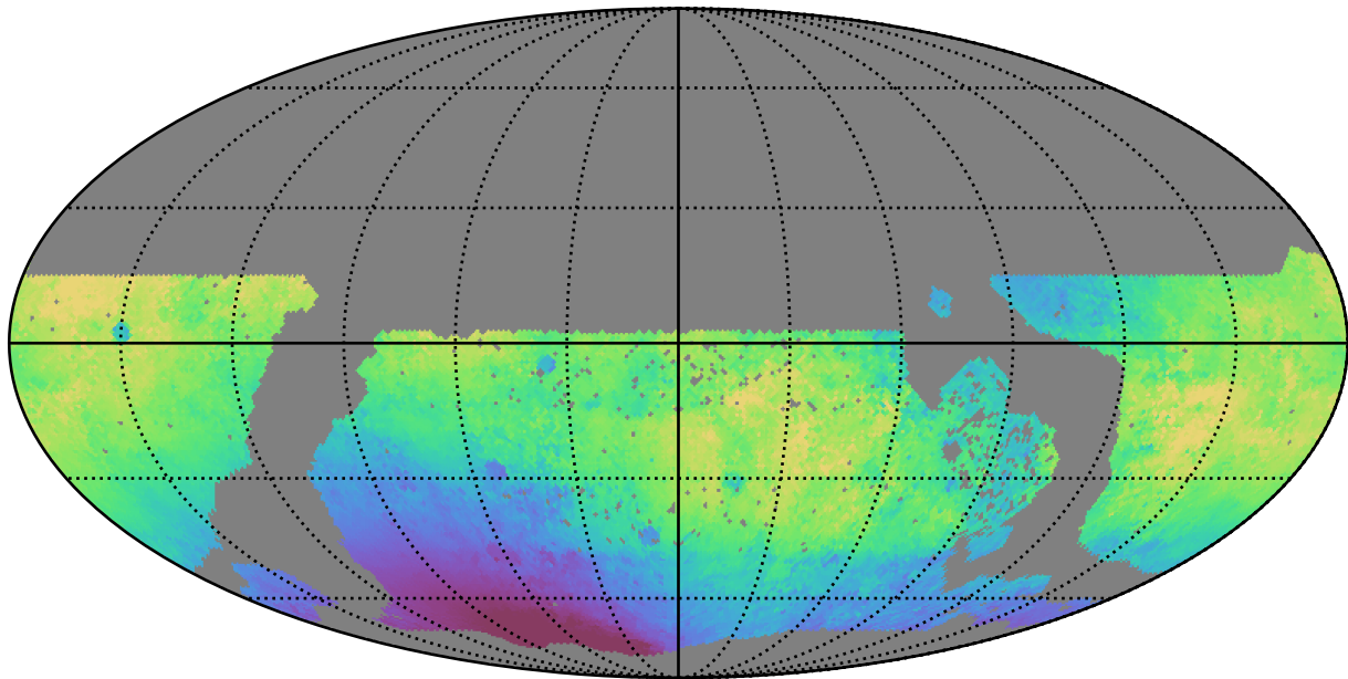
too_5_1v3.4_10yrs WFD g band: Median solarElong
