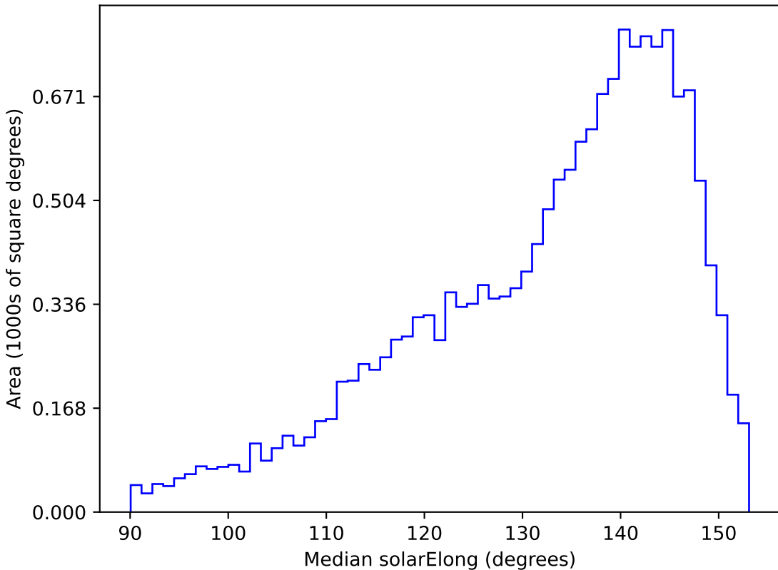
too_5_1v3.4_10yrs WFD g band: Median solarElong
