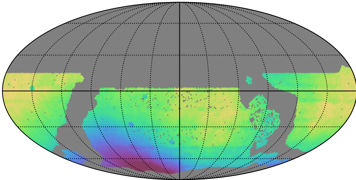
too_5_1v3.4_10yrs WFD all bands: Median solarElong
