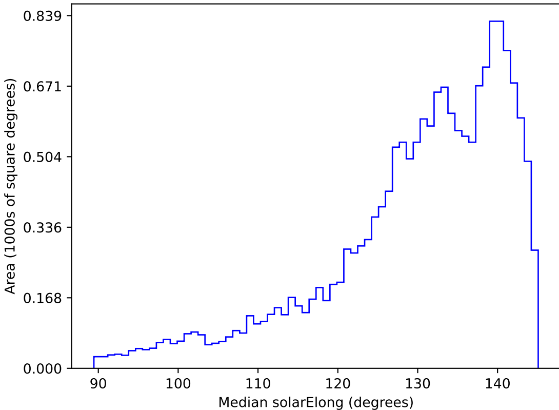
too_5_1v3.4_10yrs WFD all bands: Median solarElong
