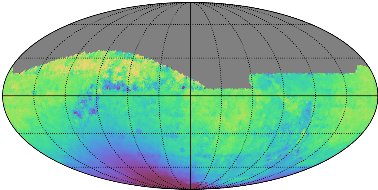
too_5_1v3.4_10yrs All sky z band: Median solarElong
