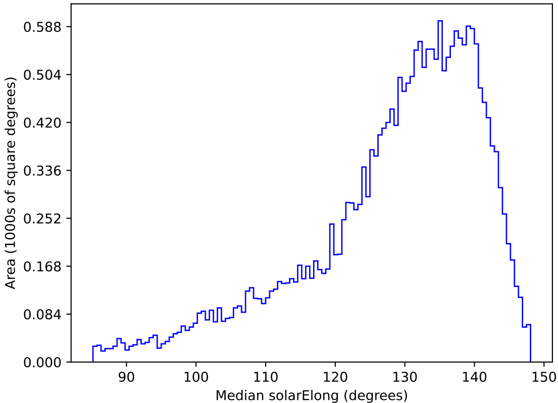
too_5_1v3.4_10yrs All sky y band: Median solarElong
