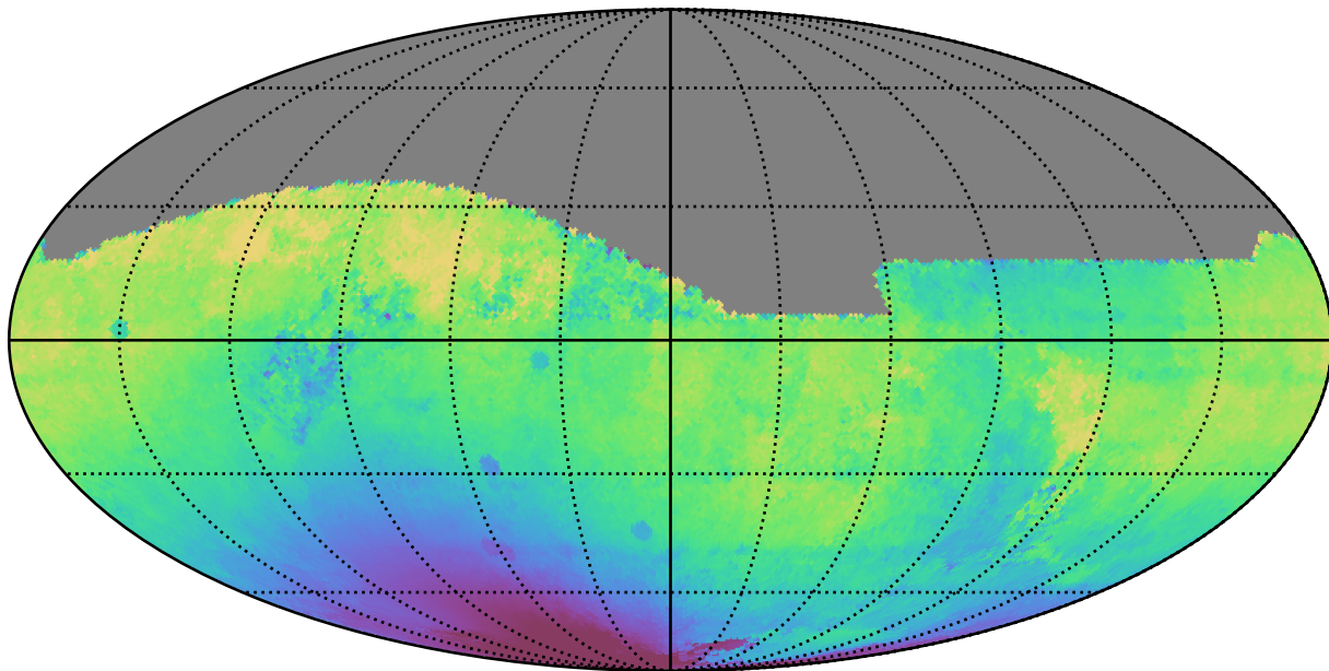
too_5_1v3.4_10yrs All sky r band: Median solarElong
